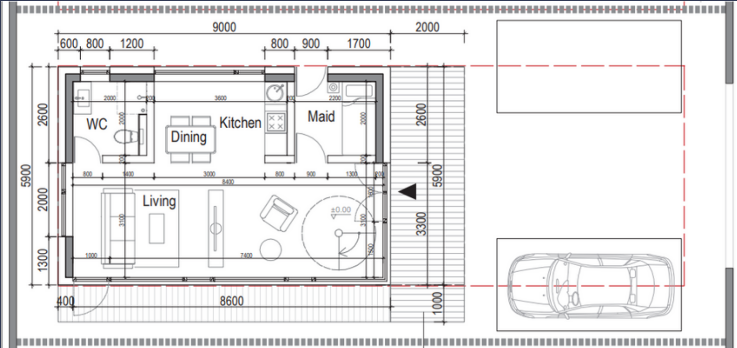
Ground floor
