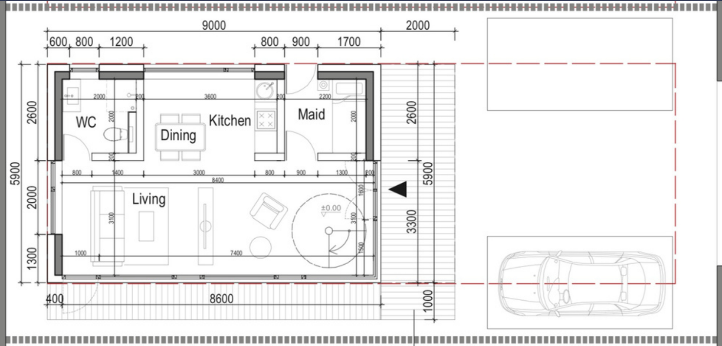
Basement parking
