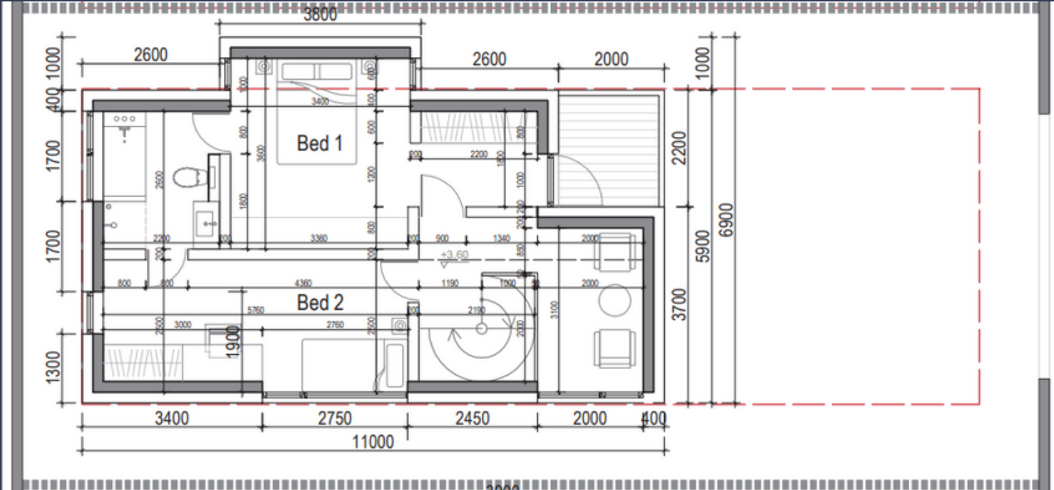
First floor
